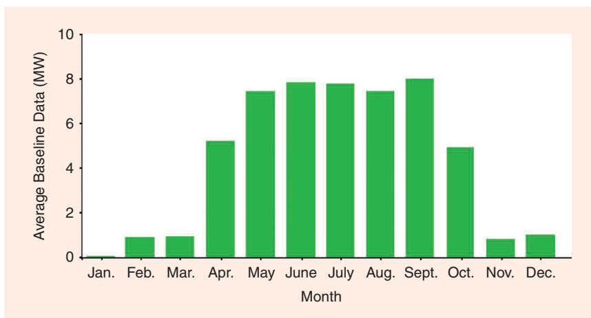
Figure 4. The power request estimation on Bersaglieri pier.
