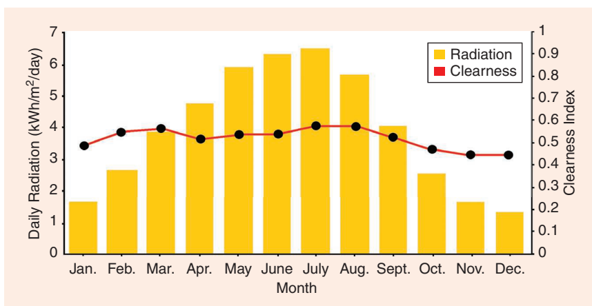
Figure 5. The daily radiation and clearness on Bersaglieri pier.
