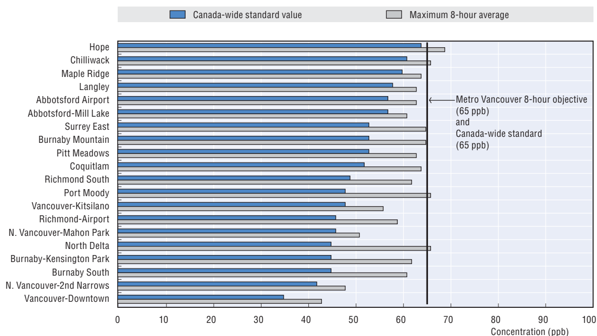
Figure 2.5. Ground-level ozone concentrations for stations in the Lower Fraser Valley
